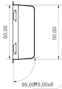
B-B (1:1)
