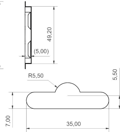
C-C (1:1)
